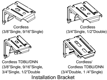
Installation Bracket
